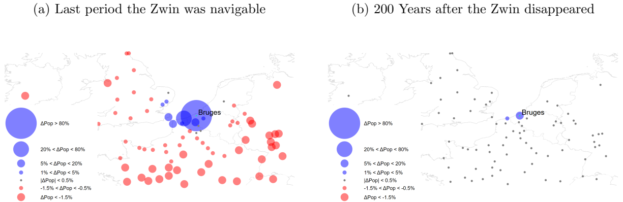
Figure 7 The model implied impact of the Zwin over space
